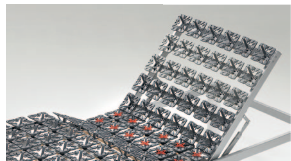
2-motors version with straight head section and attached tension clips
